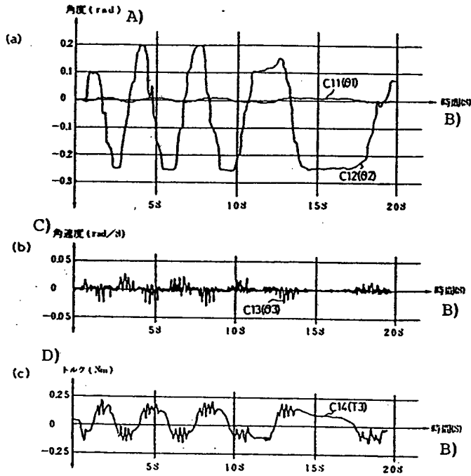
Figure 8 Key: A) Angle (rad); B) Time (S); C) Angle speed (rad/S); D) Torque (Nm).
